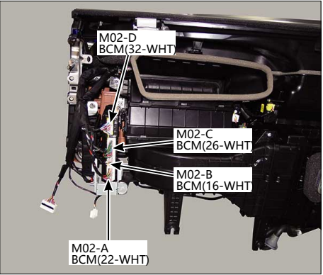
69.仪表板后右
