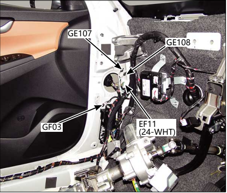
72.仪表板左侧
