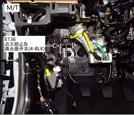
71.仪表板左侧
